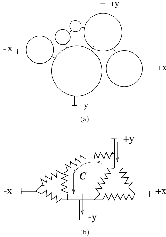
Fig. 4. (a) Typical puddle network, where dotted lines represent constrictions. (b) Corresponding equivalent circuit. Path C is denoted by arrows. [Figure taken from Ref. 25.]
