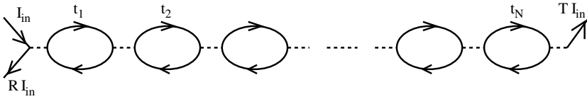
Fig. 8. A serial chain of scatterers in a Hall bar.
