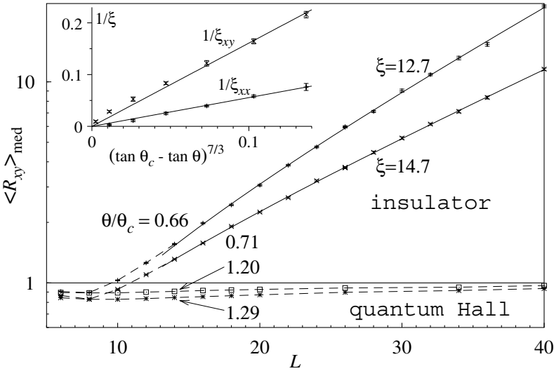
Fig. 5. Finite size scaling of the Hall resistance in the QH and insulator phases. \xi denotes the localization length, where \xi_{xx} and \xi_{xy} correspond to \rho_{xx} and \rho_{xy} , respectively. [Figure taken from Ref. 26.]
