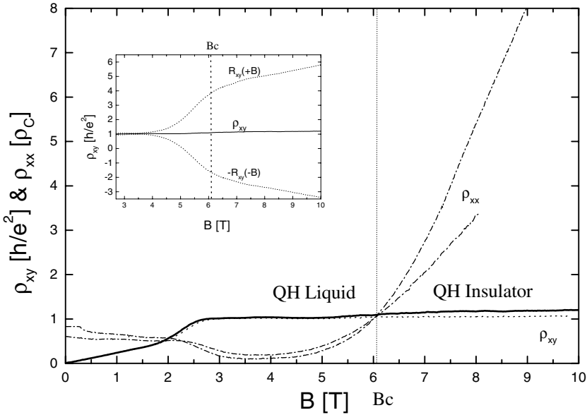
Fig. 2. The Hall and diagonal resistivities as a function of B -field. The solid line is the Hall resistivity measured at T = 300 mK and a current I = 200 nA, whereas the dotted line is for I = 400 nA. The dash-dotted lines are \rho_{xx} at T = 1.2 K (the uppermost curve) and at T = 4.2 K (the lower curve). V_G = 5.2 V, \rho_c = 1.65h/e^2 and B_C = 6.06 T. The inset shows the Hall resistances for +B and -B in dotted lines and \rho_{xy} with a solid line. [Figure taken from Ref. 17.]
