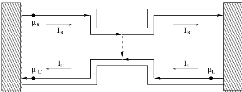
Fig. 3. A schematic illustration of a Hall bar connected to two reservoirs (shaded regions).
