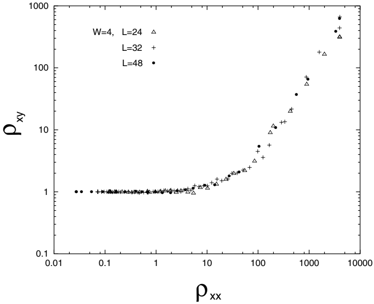
Fig. 6. \rho_{xy} versus \rho_{xx} for fixed disorder strength (denoted by W ). [Figure taken from Ref. 27.]
