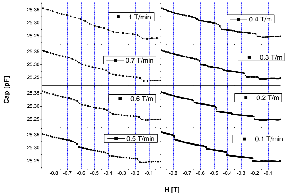
Figure 4-2: Capacitance Vs. Magnetic field at base temperature with different sweep rates.
