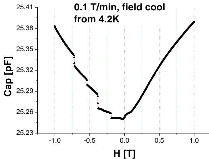
Figure 4-1: Capacitance Vs. Magnetic field at base temperature. The slope in the positive magnetic field is due to the gradient from the external field. The clear steps indicates the jumps in the magnetization.
