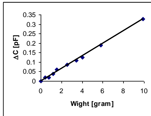
Figure 3-4 : The response of the load cell to weight at room temperature.
