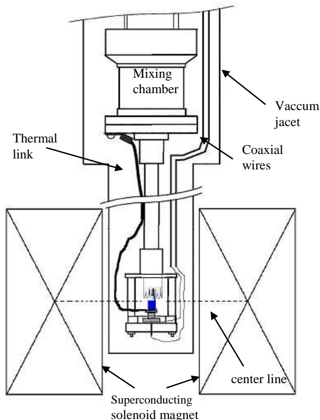
Figure 3-5 : Schematic view of the load cell device, installed off-center of a solenoid magnet in a dilution refrigerator.
