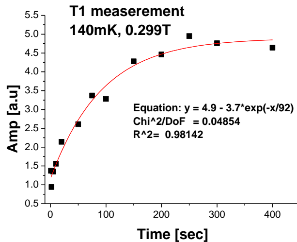
Figure 4-6: T_1 measurements for base temperature.
