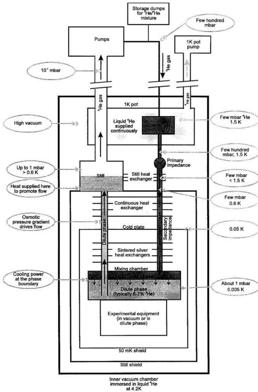
Figure 3-7: Schematic diagram of a dilution refrigerator [41].
