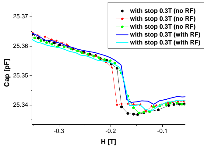
Figure 4-8: Capacitance (=Magnetization) measurement with and without RF. We saturate the nuclei and see no effect.
