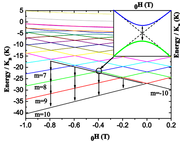
Figure 1-2: Zeeman diagram of the 21 levels of the S=10 manifold of Fe8 as a function of the field applied along the easy axis. From the bottom to the top, the levels are labeled with quantum numbers M=\pm 10, \pm 9, \dots, 0 . The inset displays in detail a two level crossing where the transverse terms (terms containing S_x and/or S_y spin operators) turn the crossing into an avoided crossing (from [12]).
