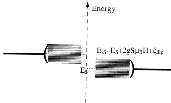
Figure 1-4: Internal dipolar fields change the energies of the two levels split by the tunnel interaction, and thus hinder tunneling. By effectively broadening the levels, hyperfine interactions restore the matching of the left and right levels, and thus allow tunneling.
