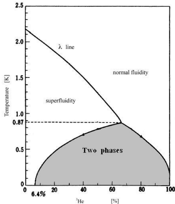
Figure 3-6: Phase diagram of ^3\text{He}/^4\text{He} [41].
