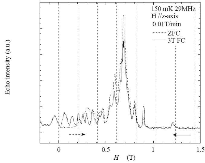
Figure 2-5: Field cool and zero field cool ^1\text{H} -NMR spectra for FE8 single crystal at 150mK 29MHz. the broken lines show calculated level crossing field. From [34]
