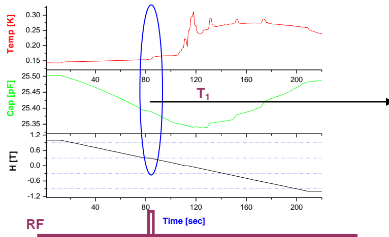
Figure 4-7: scheme of the measurements with RF. We sweep the magnetic field from positive to negative, and stop for several seconds to transmit the RF at 0.3T. We see that the temperature rise due to the transmitting is low, and the first two jumps are in the regime of the T_1 .
