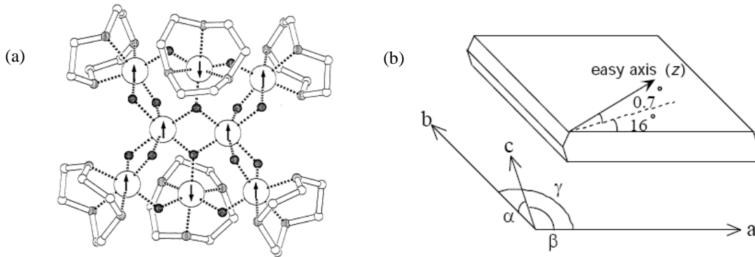
Figure 2-1: Structure of the molecular nanomagnet Fe8: (a) molecular view - the spin structure is schematized by the arrows [25]; (b) crystal shape - schematic view of the anisotropy axes and the crystal axes [12].
