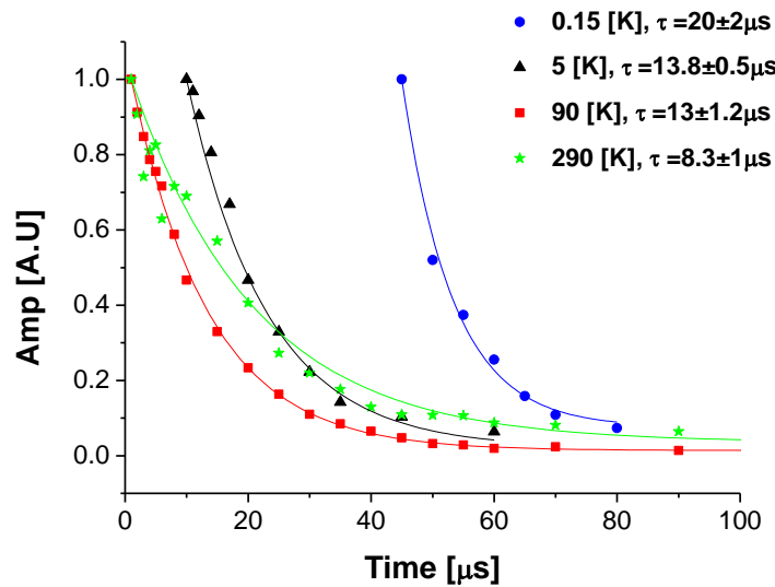
Figure 4-5: T_2 measurements for several temperatures.
