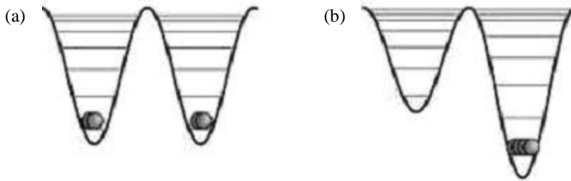
Figure 1-1: Energy levels for a spin state S with easy axis magnetic anisotropy. The +M levels are localized in the left side and the -M levels in the right side. a) In zero field the two states are equally populated; b) the application of a magnetic field selectively populates the right side.
