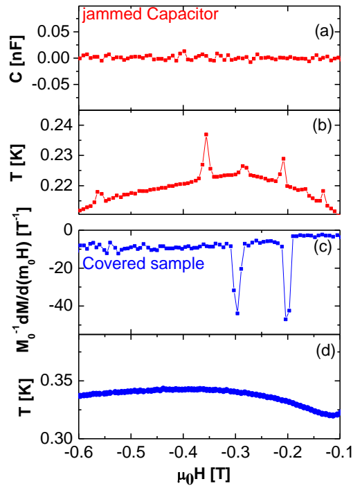
Figure 4-11: Test cases: The capacitance (a) and temperature (b) vs. magnetic field swept from positive to negative with jammed capacitor. The rise in the temperature indicates the change in the magnetization. The normalized derivative of the magnetization (c) and temperature (d) vs. magnetic field (same sweeping direction) with covered sample. The change in the magnetization is not followed this time by an increase in the temperature.
